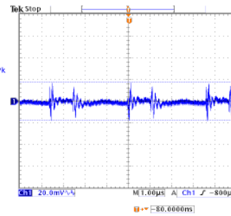
High Line, Full Load Ripple noise=35.2mV
