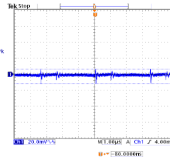
High Line, Full Load Ripple noise=18.4mV
