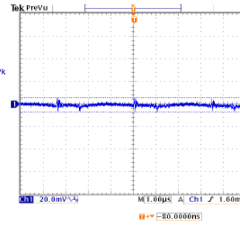
High Line, Full Load Ripple noise=12.4mV
