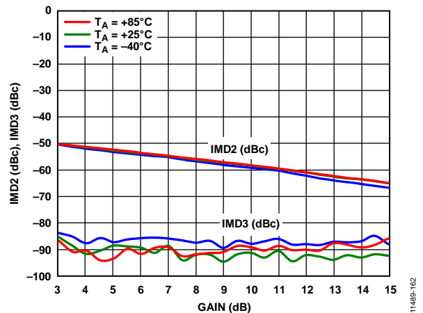
Figure 65. DGA IMD2/IMD3 vs. Gain Setting
